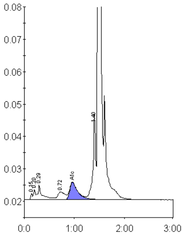
Peak table - ID: 10592884
